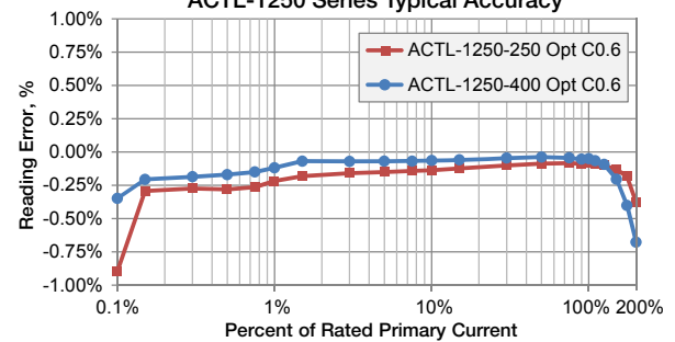
ACTL-1250 Series Typical Accuracy
