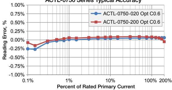
ACTL-0750 Series Typical Accuracy
