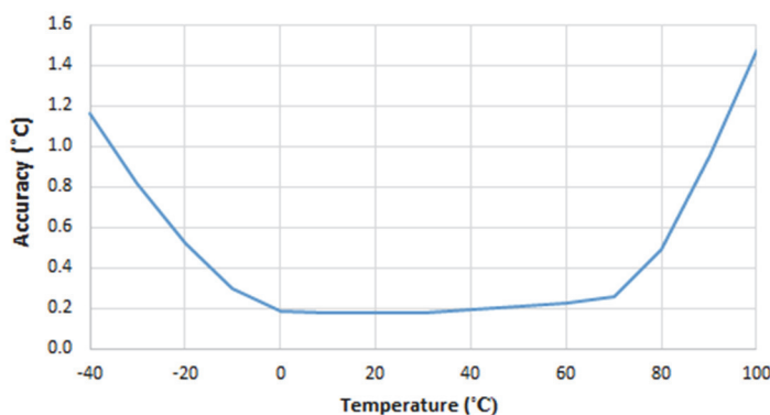
Plot A: 12-Bit Temperature Smart Sensor Accuracy
