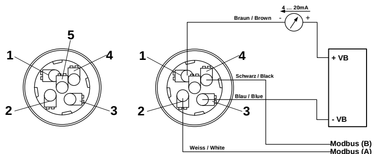
Connector plug
