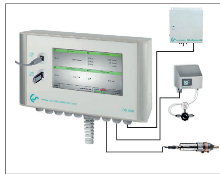
Fig. 2: DS 500 paperless recorder with PC 400, Oil check 400, FA 510 dew point sensor
