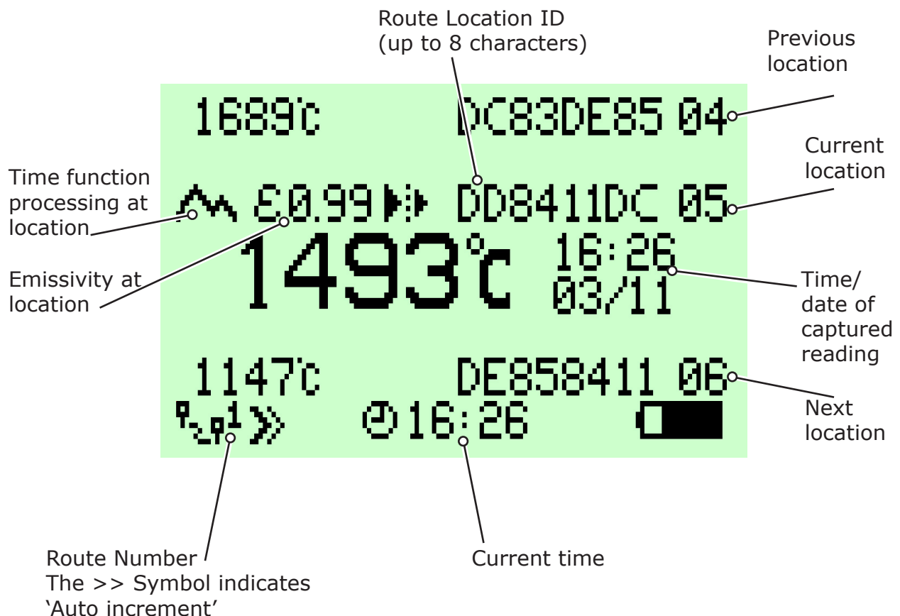
Fig. 7-5 Typical Route Mode display
