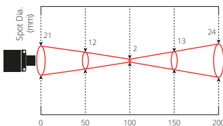
Distance: Sensor to object (mm) PCU-MA2.0
