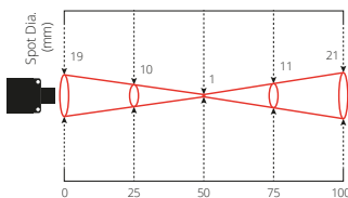
Distance: Sensor to object (mm) PCU-MA1.0
