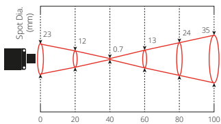
Distance: Sensor to object (mm) PCU-XSA0.7
