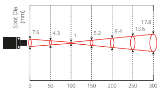
Distance: Sensor to object (mm) PCU-XSB1.0
