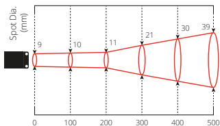
Distance: Sensor to object (mm) PCU-MB11.0
