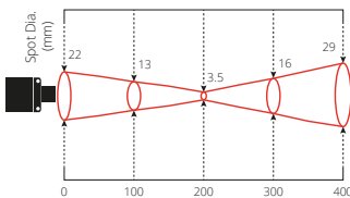
Distance: Sensor to object (mm) PCU-MA3.5
