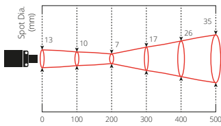
Distance: Sensor to object (mm) PCU-F7.0
