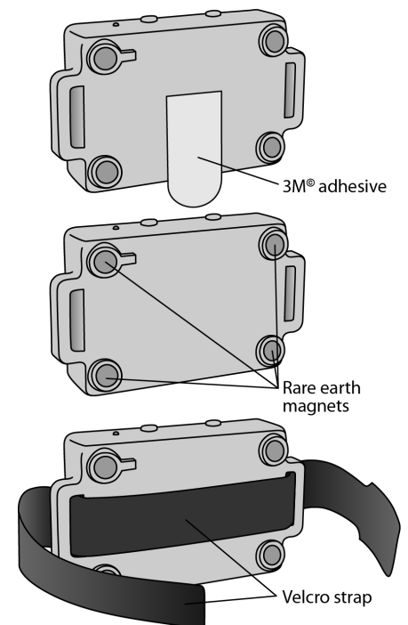
Data logger securing methods
